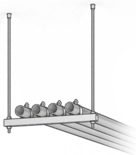
Trapeze-supported pipes
